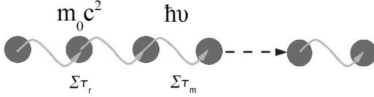
Figure 1: The schema of the separation in time and space the wave ( \hbar\nu ; \sum \tau_m ; \sum L_m ) and particle ( m_0c^2 ; \sum \tau_r ) properties of micro-objects.
